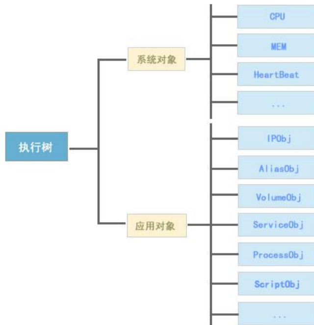
Execute Tree Model
