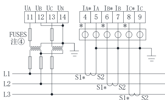
3P3i/2PT+3CT (仪表设置为3P3i) 注③
