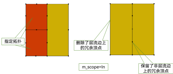
图 9-23 m_scope=In
