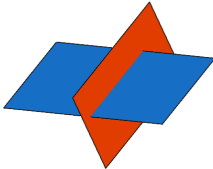
干涉 (interference)
