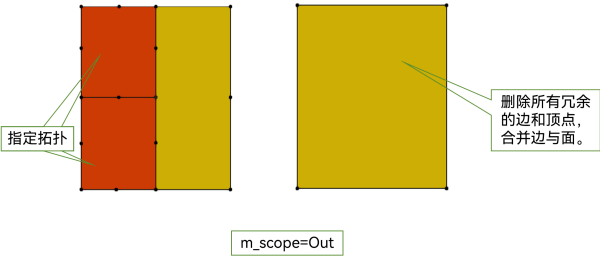
图 9-25 m_scope=Out
