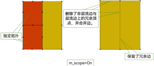
图 9-24 m_scope=On
